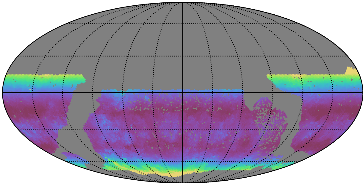
no_high_blob_v3.3_10yrs WFD g band: Median airmass
