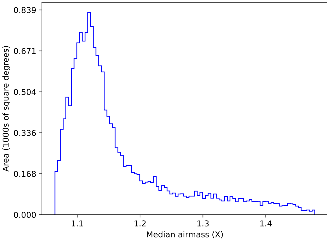
no_high_blob_v3.3_10yrs WFD g band: Median airmass
