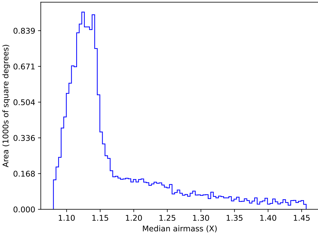
no_high_blob_v3.3_10yrs WFD all bands: Median airmass
