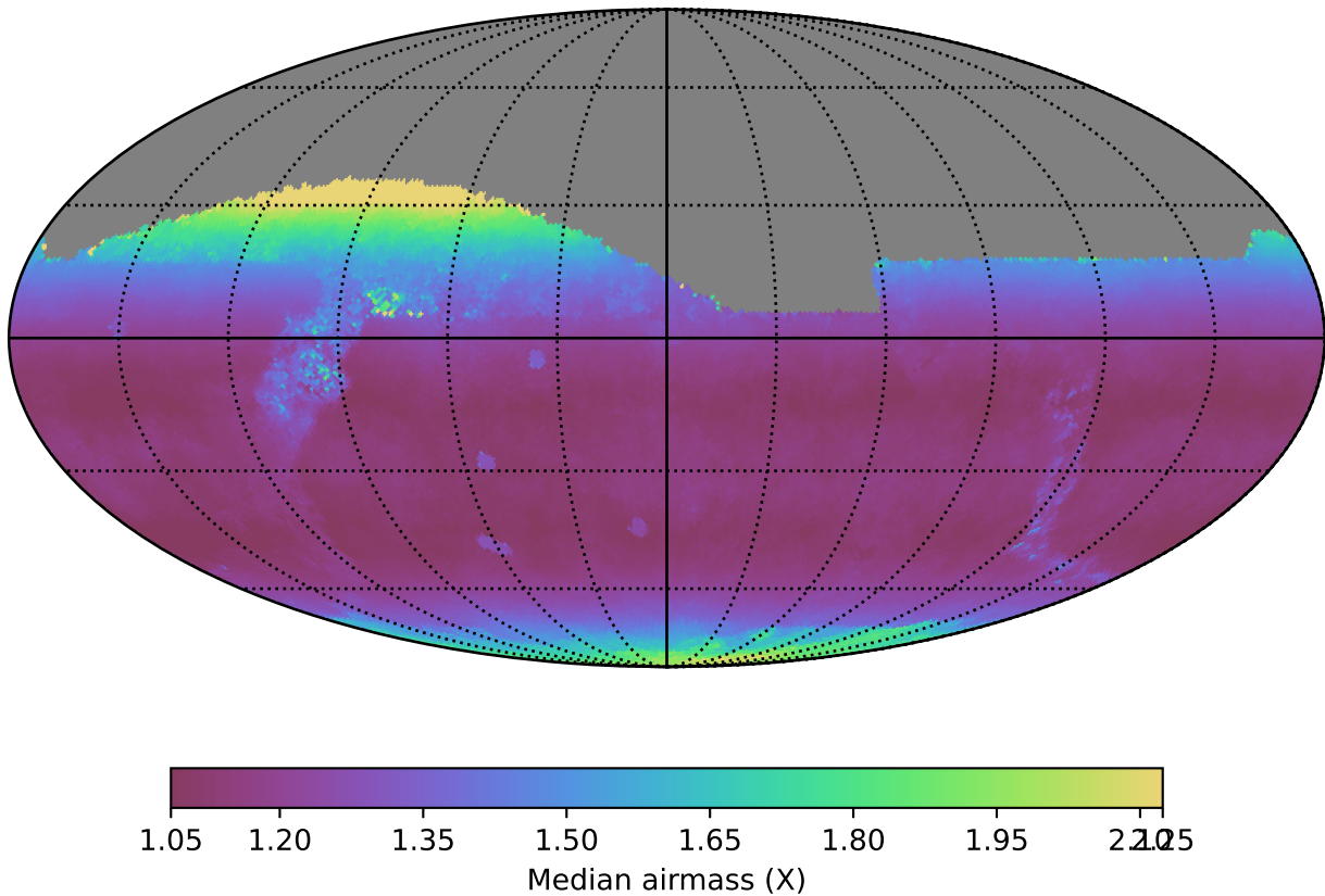
no_high_blob_v3.3_10yrs All sky z band: Median airmass
