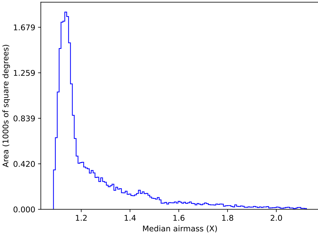
no_high_blob_v3.3_10yrs All sky z band: Median airmass
