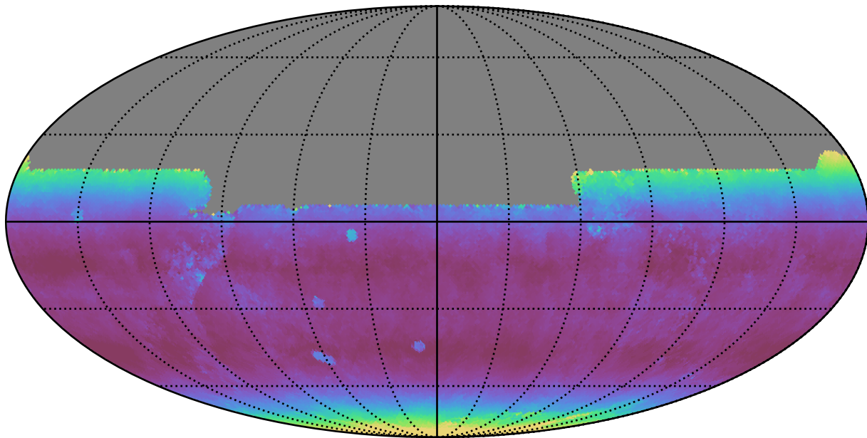
no_high_blob_v3.3_10yrs All sky y band: Median airmass
