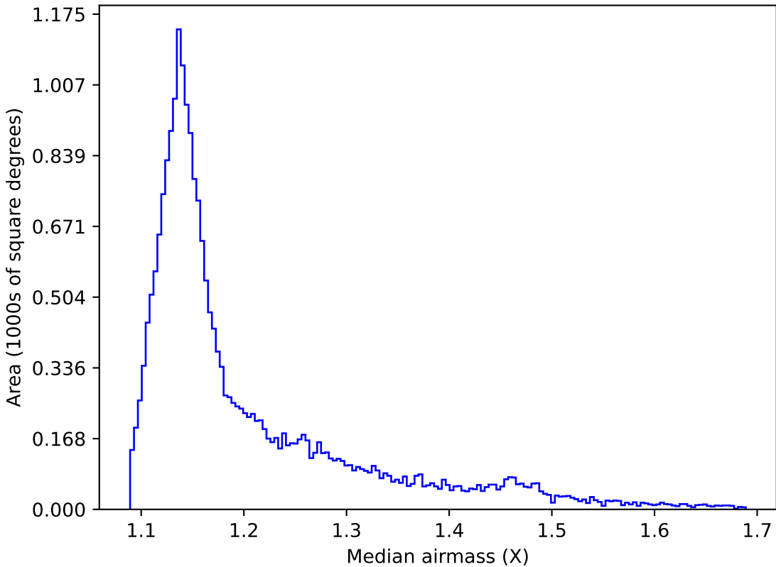
no_high_blob_v3.3_10yrs All sky y band: Median airmass
