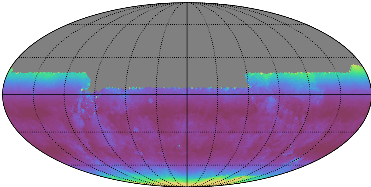
no_high_blob_v3.3_10yrs All sky u band: Median airmass
