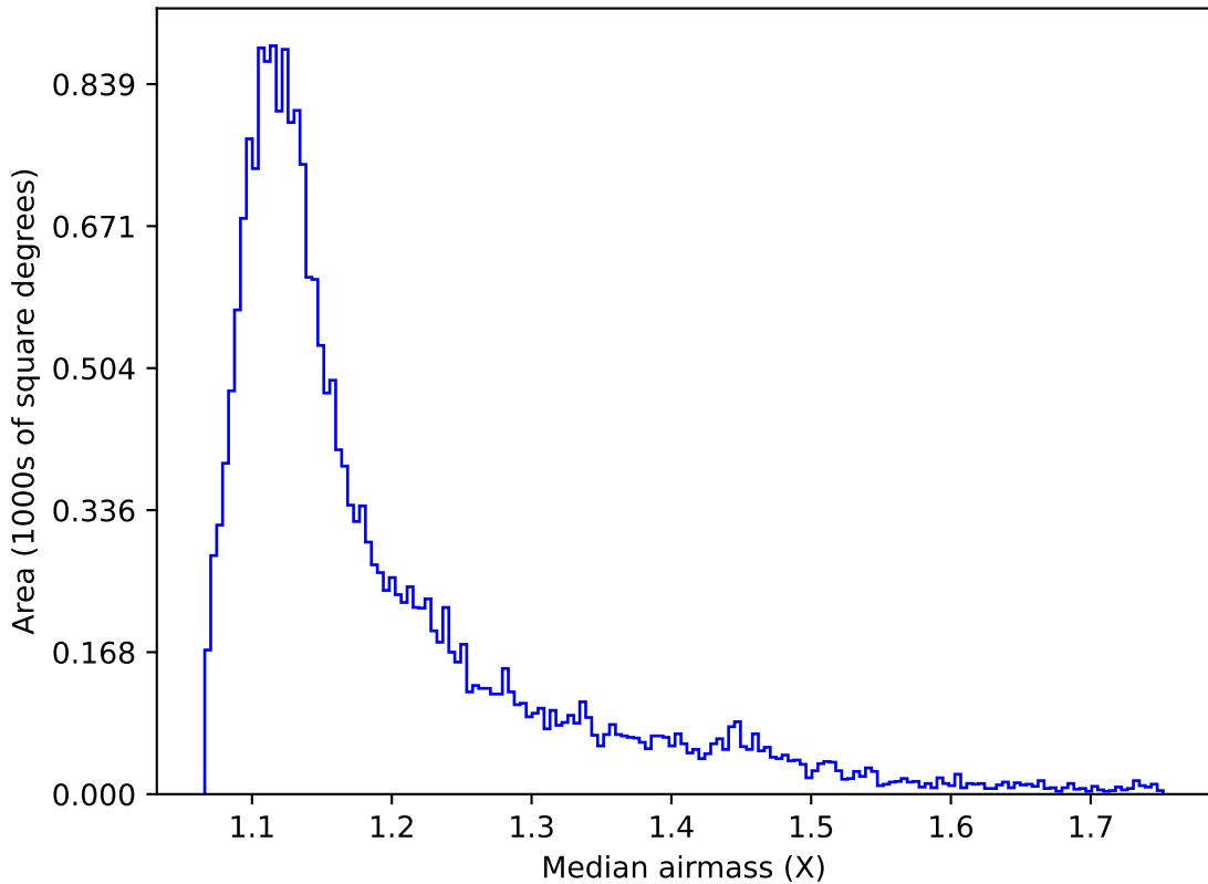
no_high_blob_v3.3_10yrs All sky u band: Median airmass
