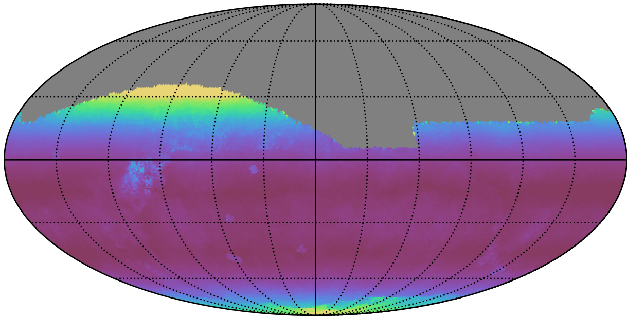
no_high_blob_v3.3_10yrs All sky r band: Median airmass
