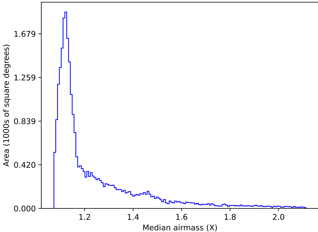
no_high_blob_v3.3_10yrs All sky r band: Median airmass
