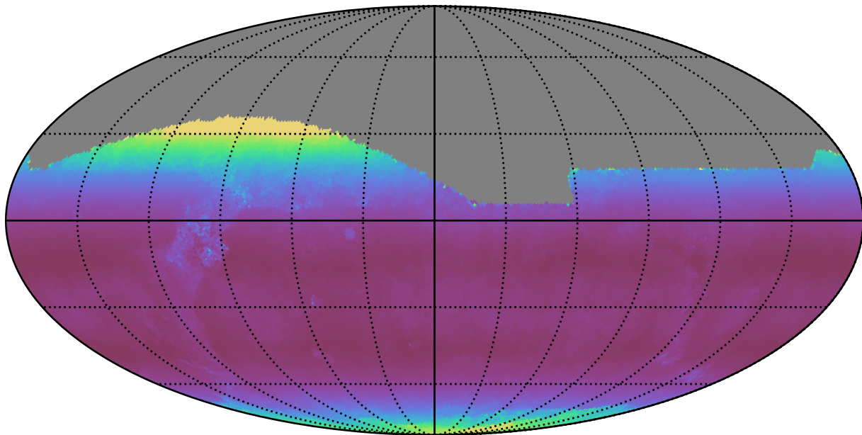
no_high_blob_v3.3_10yrs All sky i band: Median airmass
