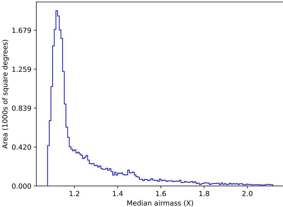
no_high_blob_v3.3_10yrs All sky i band: Median airmass
