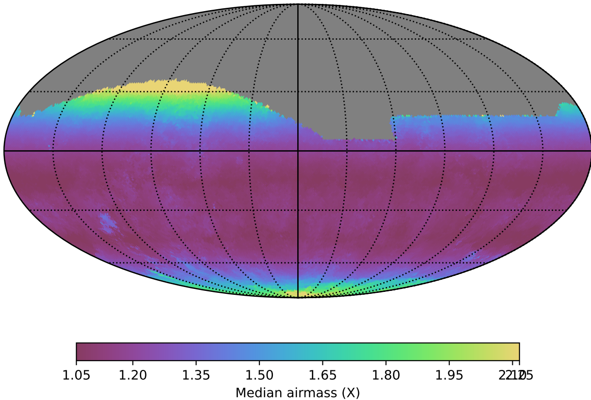
no_high_blob_v3.3_10yrs All sky g band: Median airmass
