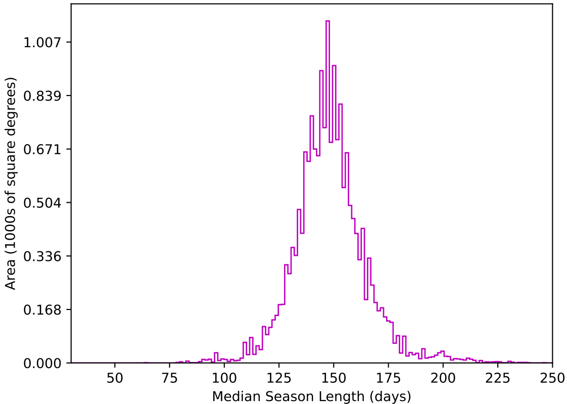
no_high_blob_v3.3_10yrs WFD z band: Median Season Length
