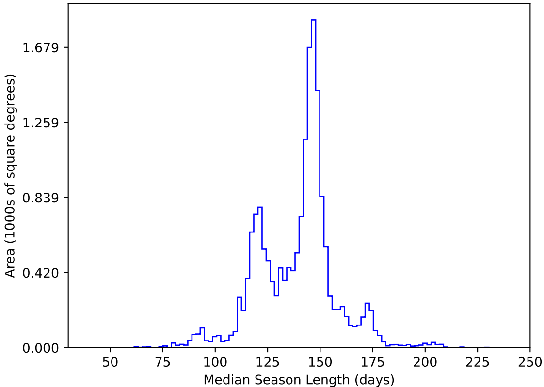
no_high_blob_v3.3_10yrs WFD y band: Median Season Length
