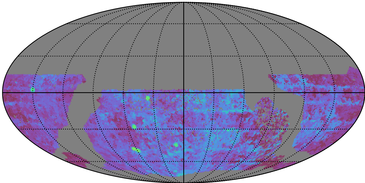
no_high_blob_v3.3_10yrs WFD u band: Median Season Length
