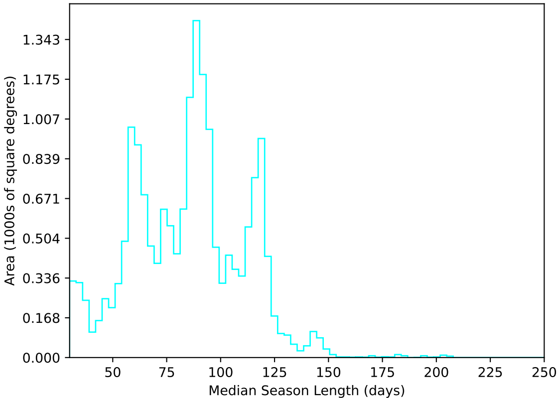
no_high_blob_v3.3_10yrs WFD u band: Median Season Length
