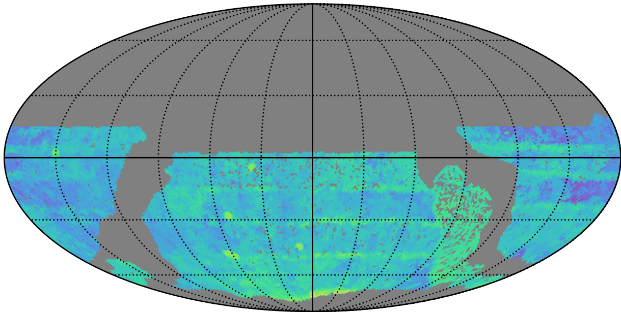
no_high_blob_v3.3_10yrs WFD r band: Median Season Length
