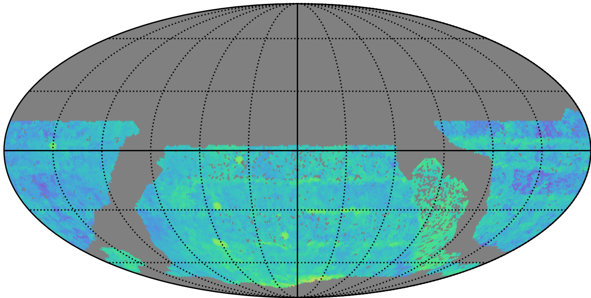
no_high_blob_v3.3_10yrs WFD i band: Median Season Length
