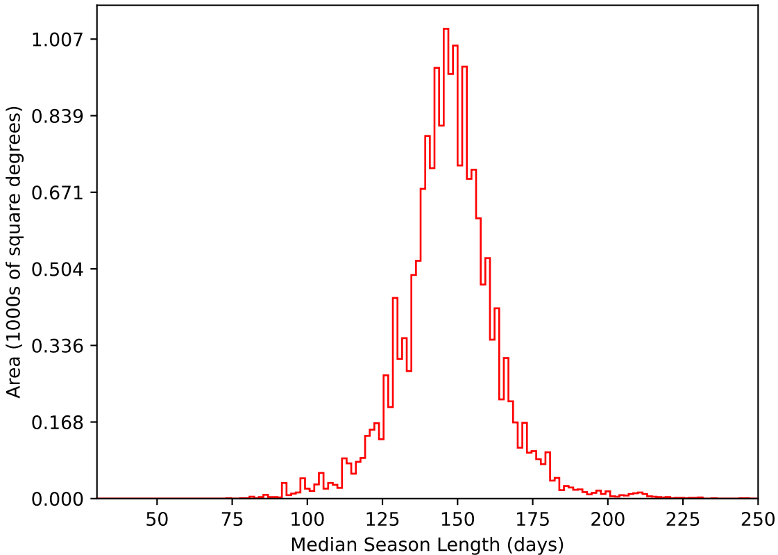
no_high_blob_v3.3_10yrs WFD i band: Median Season Length
