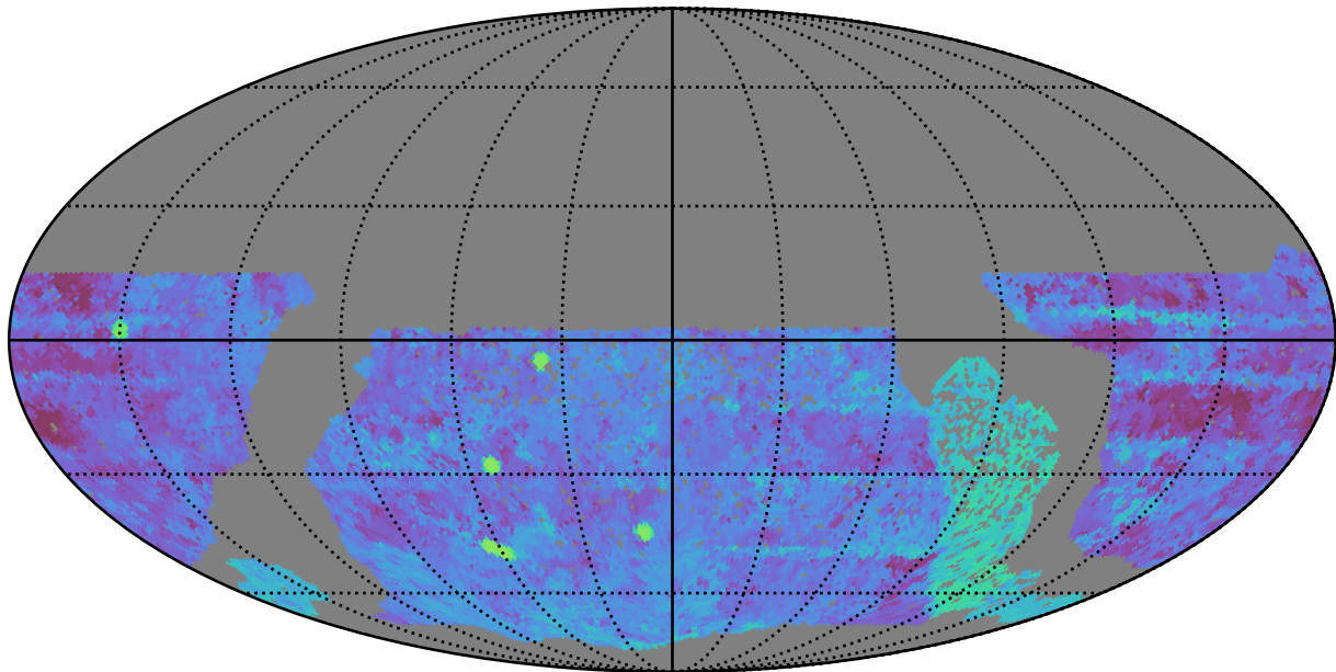
no_high_blob_v3.3_10yrs WFD g band: Median Season Length
