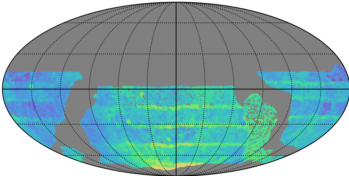
no_high_blob_v3.3_10yrs WFD all bands: Median Season Length
