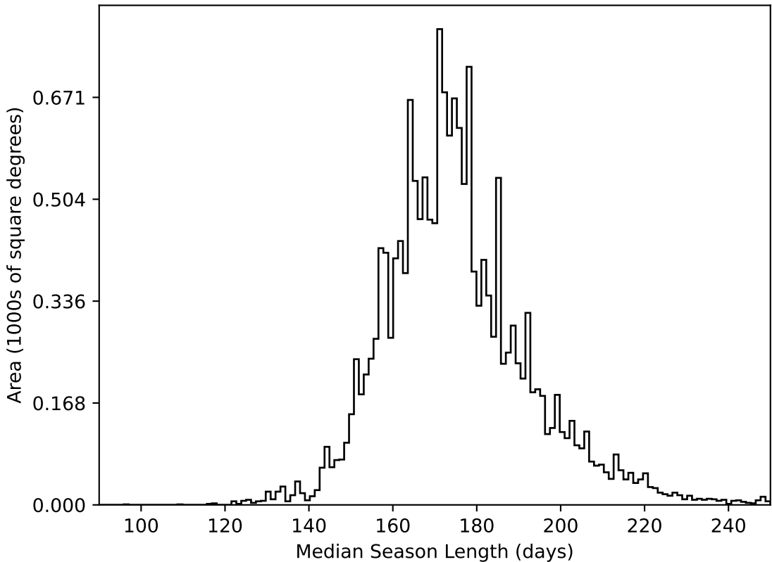
no_high_blob_v3.3_10yrs WFD all bands: Median Season Length
