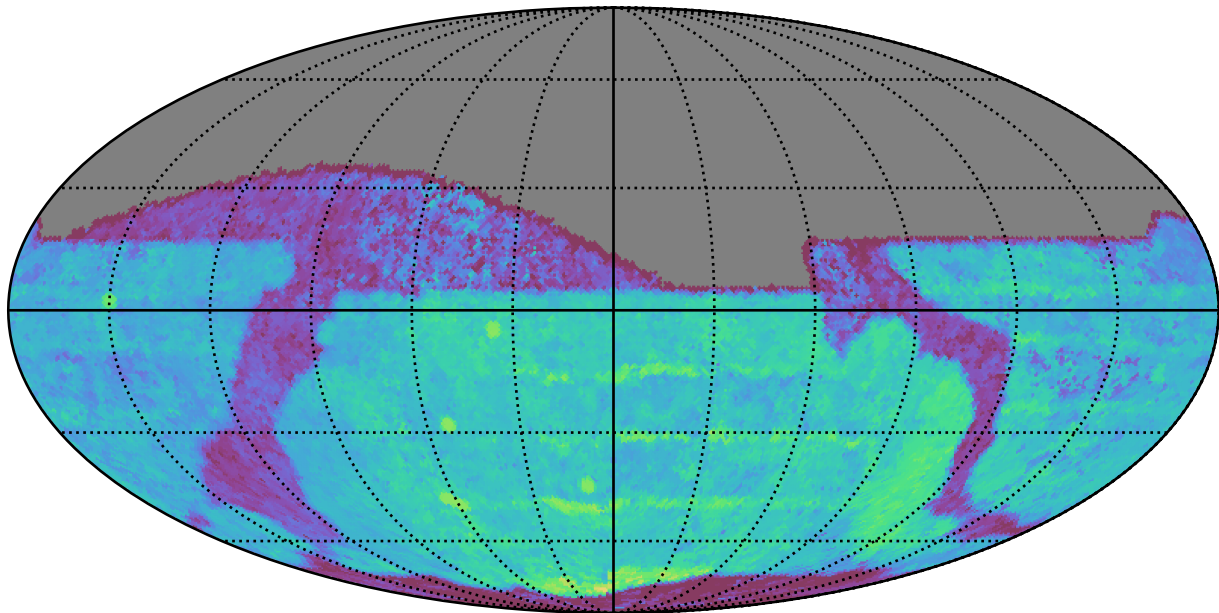
no_high_blob_v3.3_10yrs All sky z band: Median Season Length
