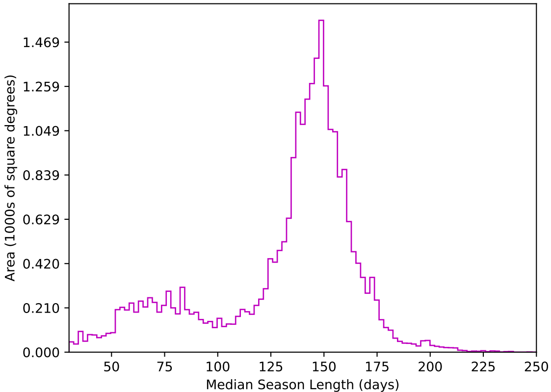
no_high_blob_v3.3_10yrs All sky z band: Median Season Length
