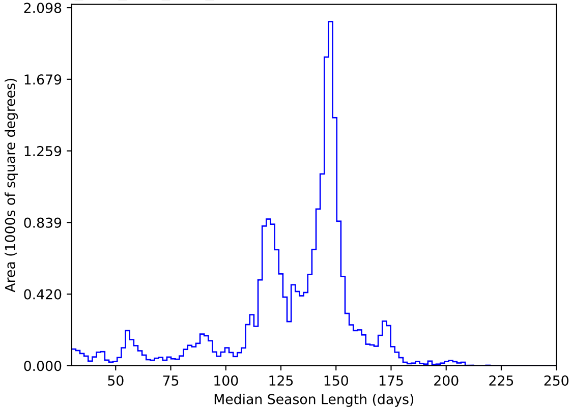
no_high_blob_v3.3_10yrs All sky y band: Median Season Length
