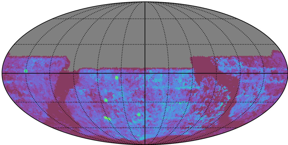
no_high_blob_v3.3_10yrs All sky u band: Median Season Length
