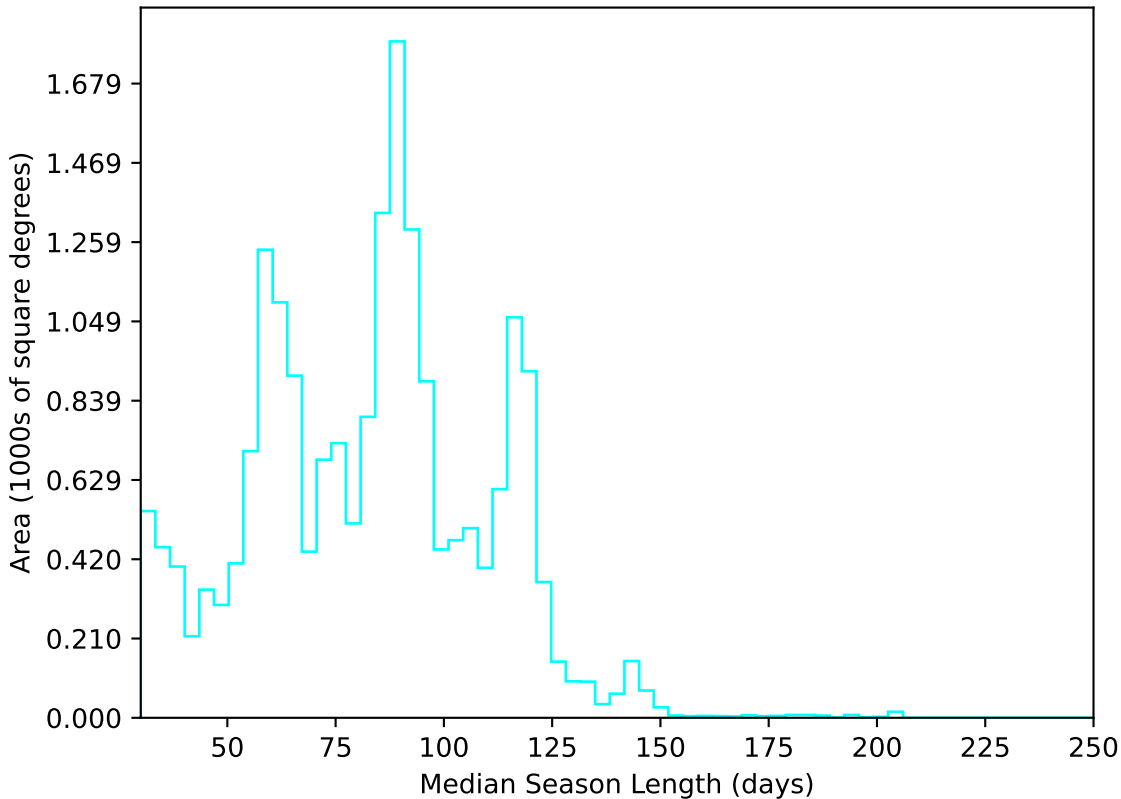
no_high_blob_v3.3_10yrs All sky u band: Median Season Length
