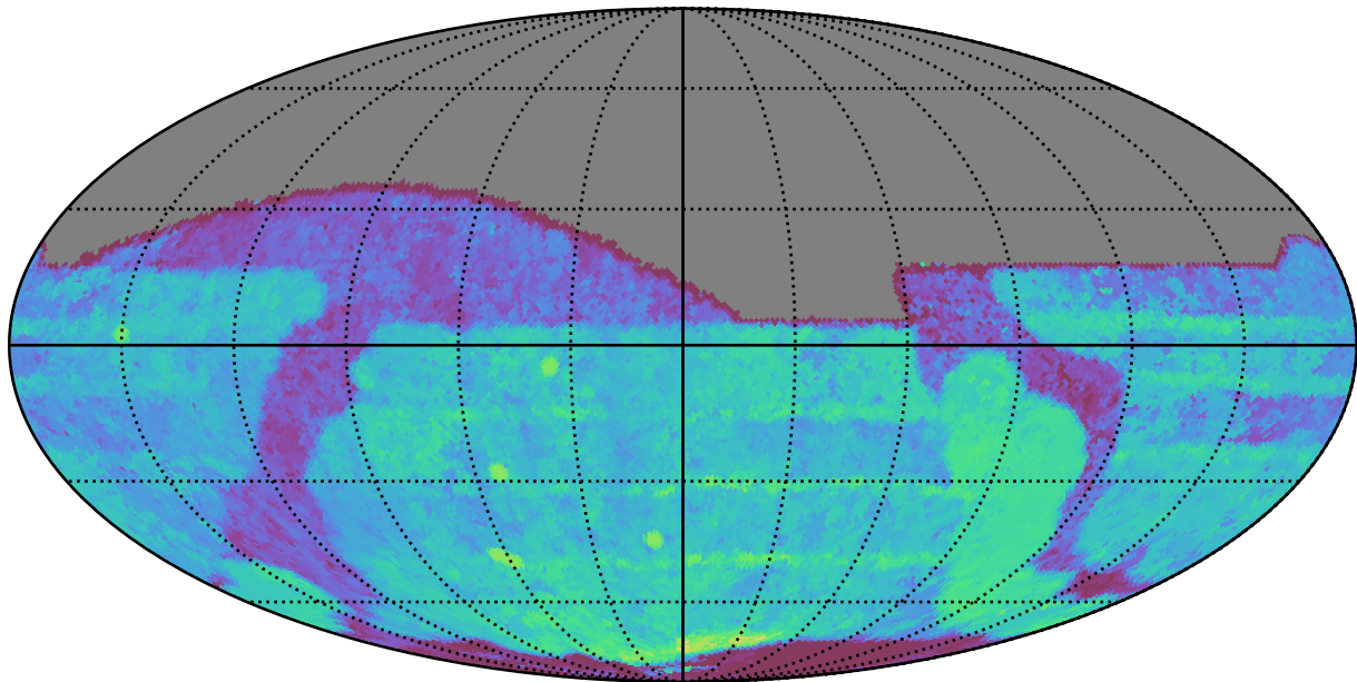
no_high_blob_v3.3_10yrs All sky r band: Median Season Length
