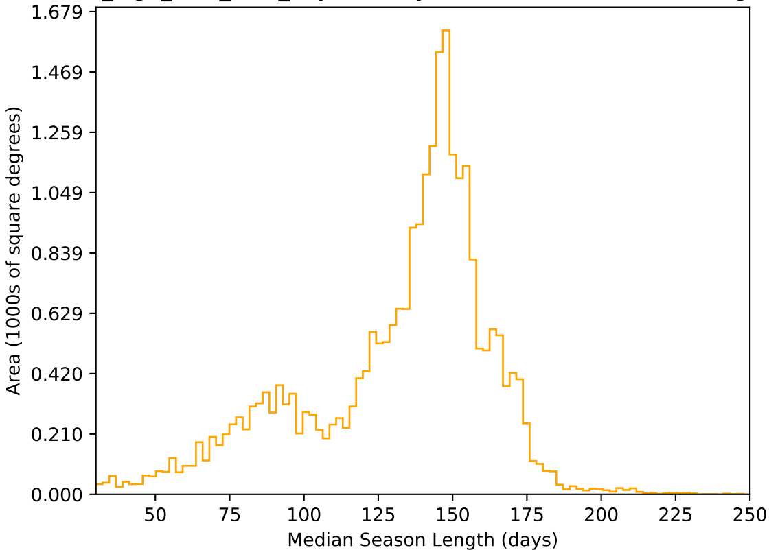
no_high_blob_v3.3_10yrs All sky r band: Median Season Length
