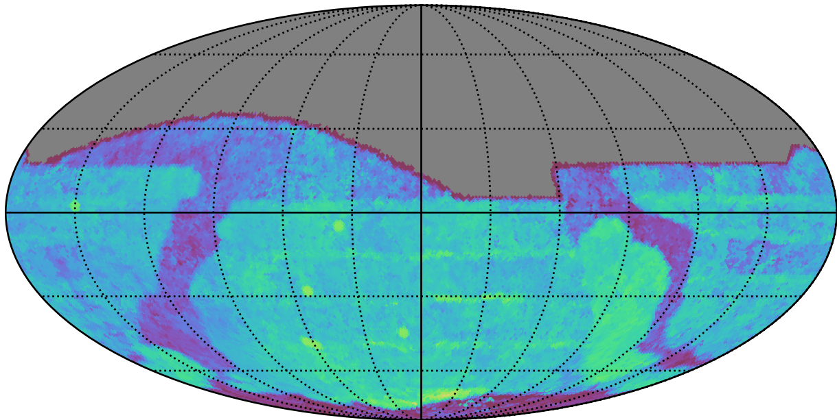
no_high_blob_v3.3_10yrs All sky i band: Median Season Length
