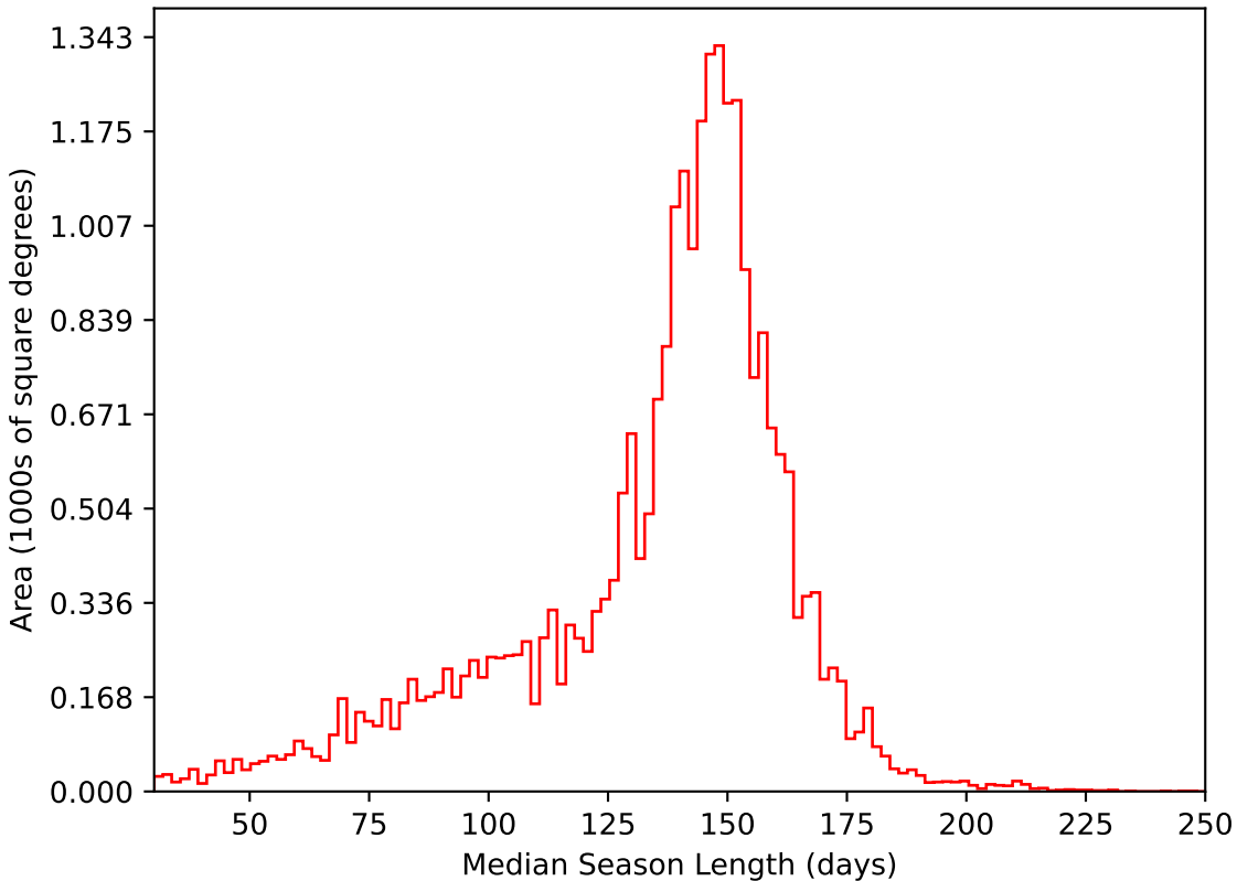
no_high_blob_v3.3_10yrs All sky i band: Median Season Length
