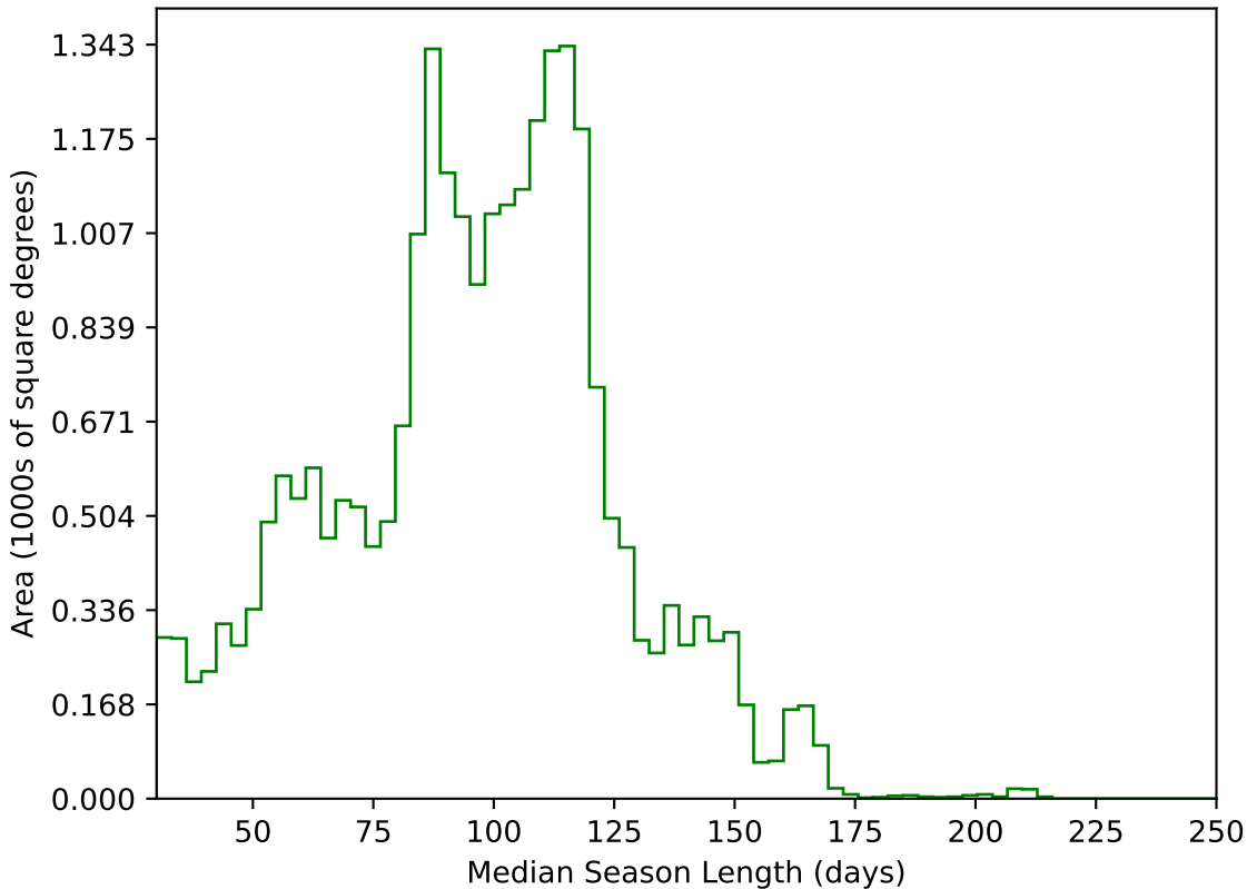
no_high_blob_v3.3_10yrs All sky g band: Median Season Length
