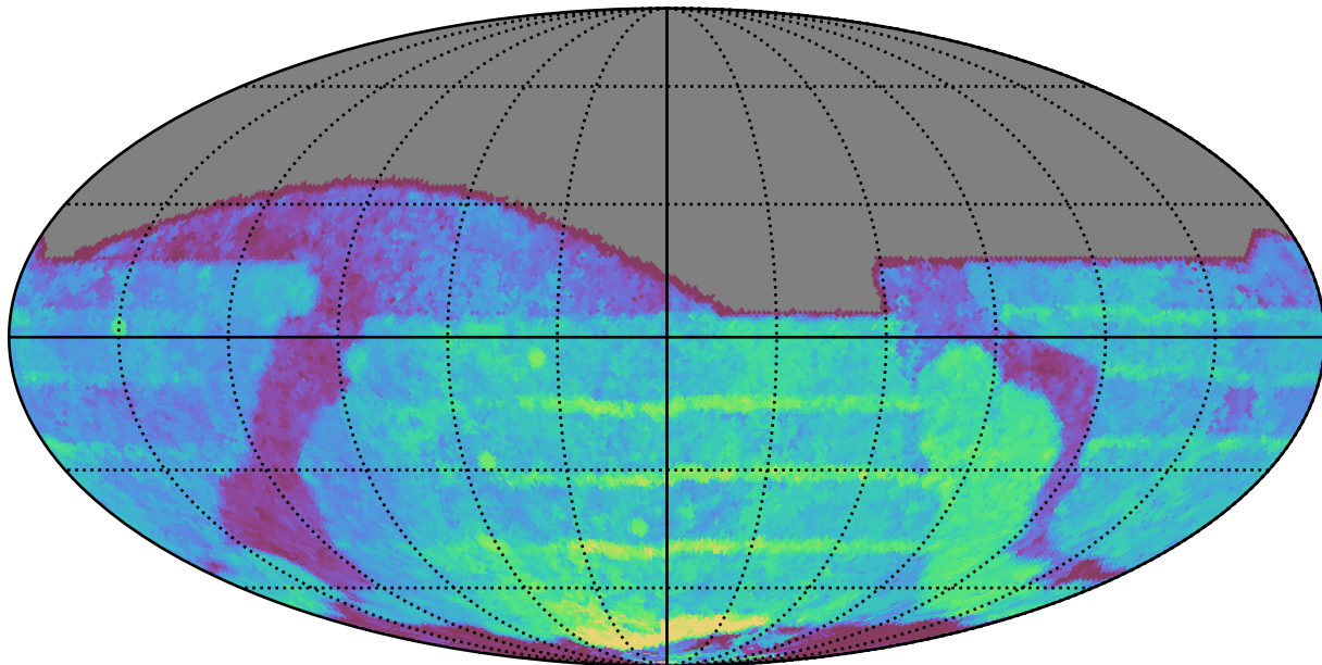
no_high_blob_v3.3_10yrs All sky all bands: Median Season Length
