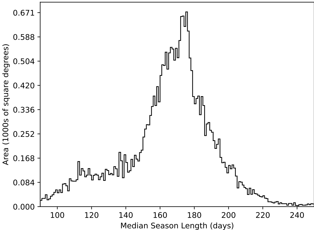
no_high_blob_v3.3_10yrs All sky all bands: Median Season Length
