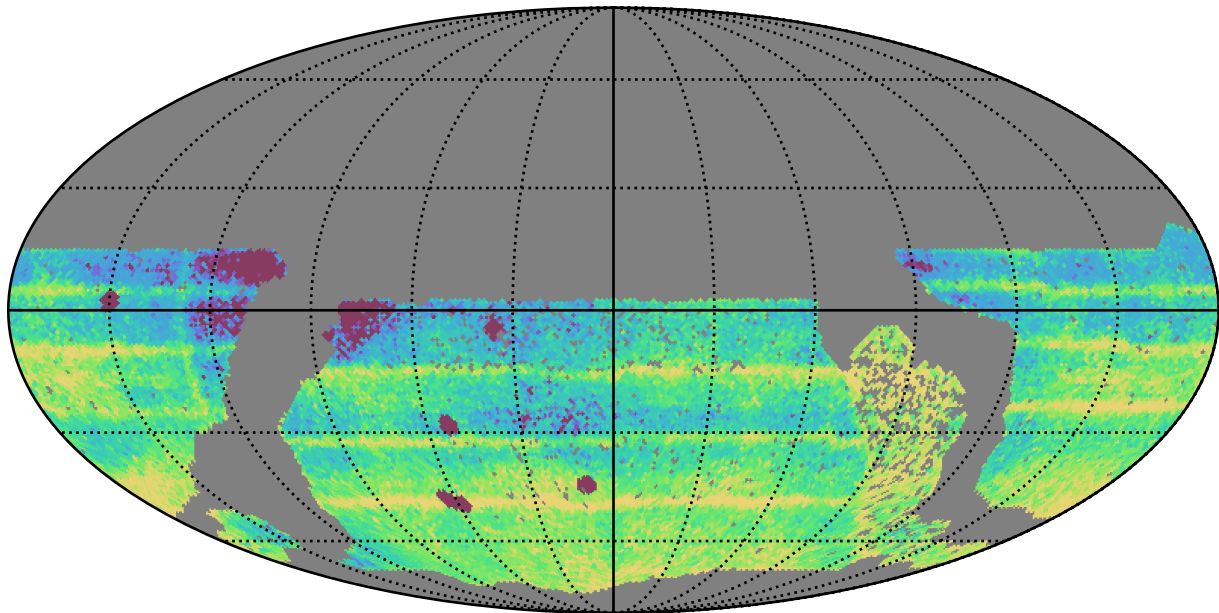
no_high_blob_v3.3_10yrs WFD: Median Intra-Night Gap
