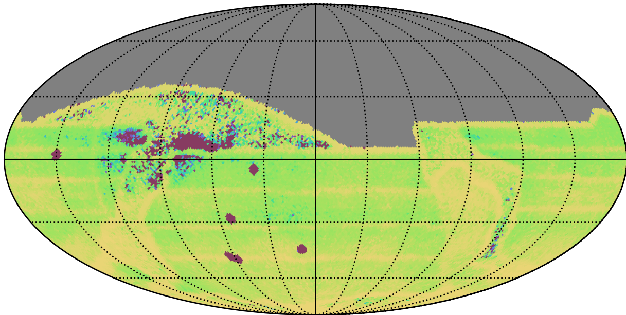
no_high_blob_v3.3_10yrs All sky: Median Intra-Night Gap
