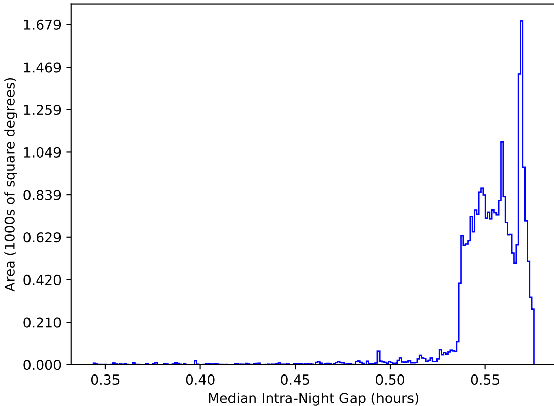
no_high_blob_v3.3_10yrs All sky: Median Intra-Night Gap
