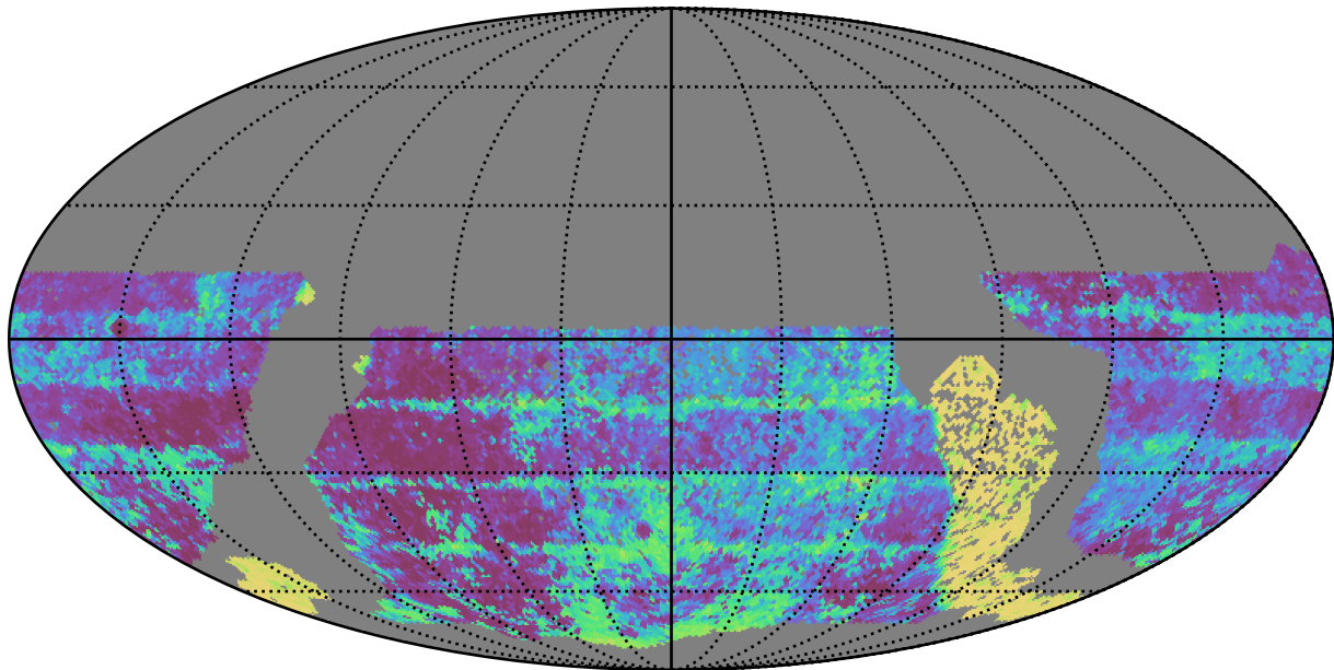
no_high_blob_v3.3_10yrs WFD y band: Median Inter-Night Gap
