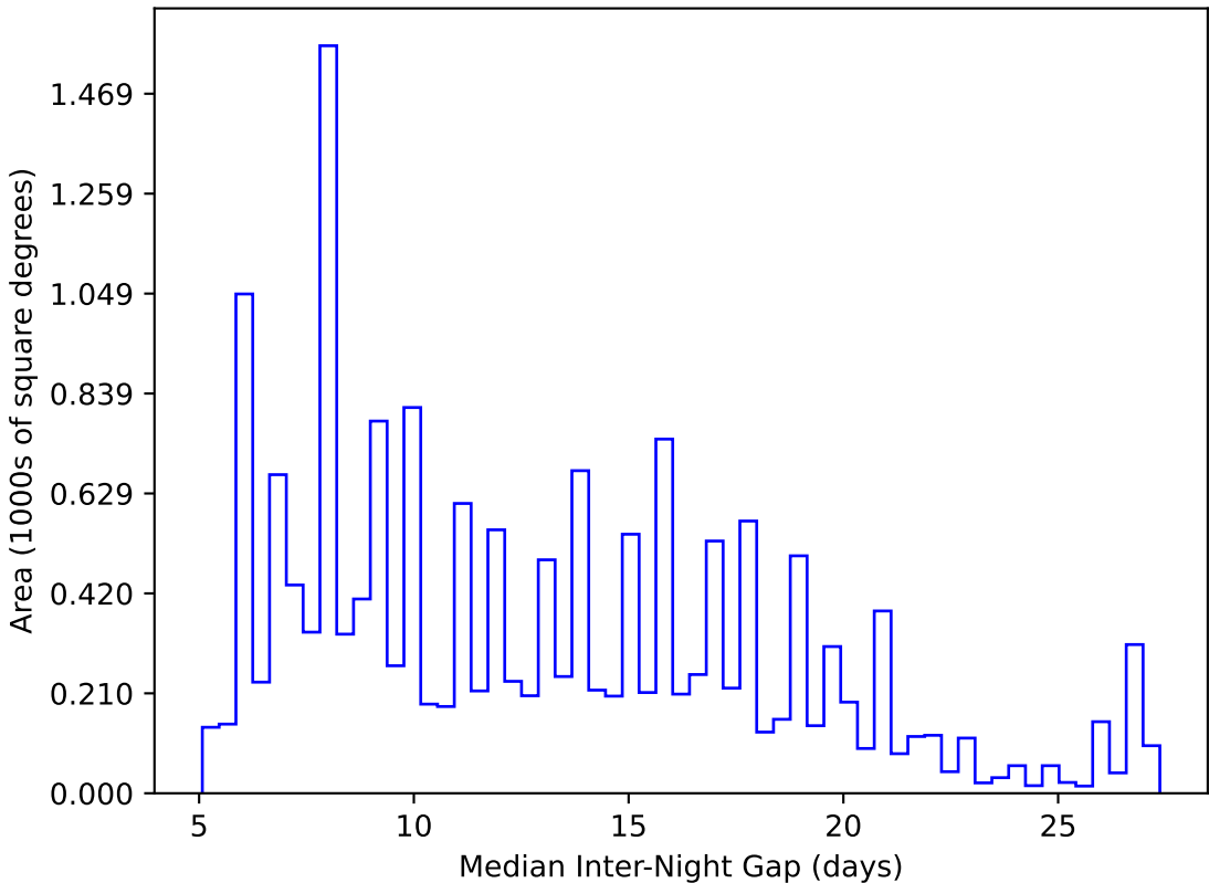
no_high_blob_v3.3_10yrs WFD y band: Median Inter-Night Gap
