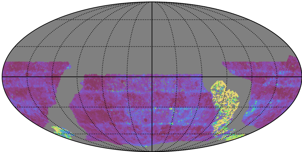
no_high_blob_v3.3_10yrs WFD u band: Median Inter-Night Gap
