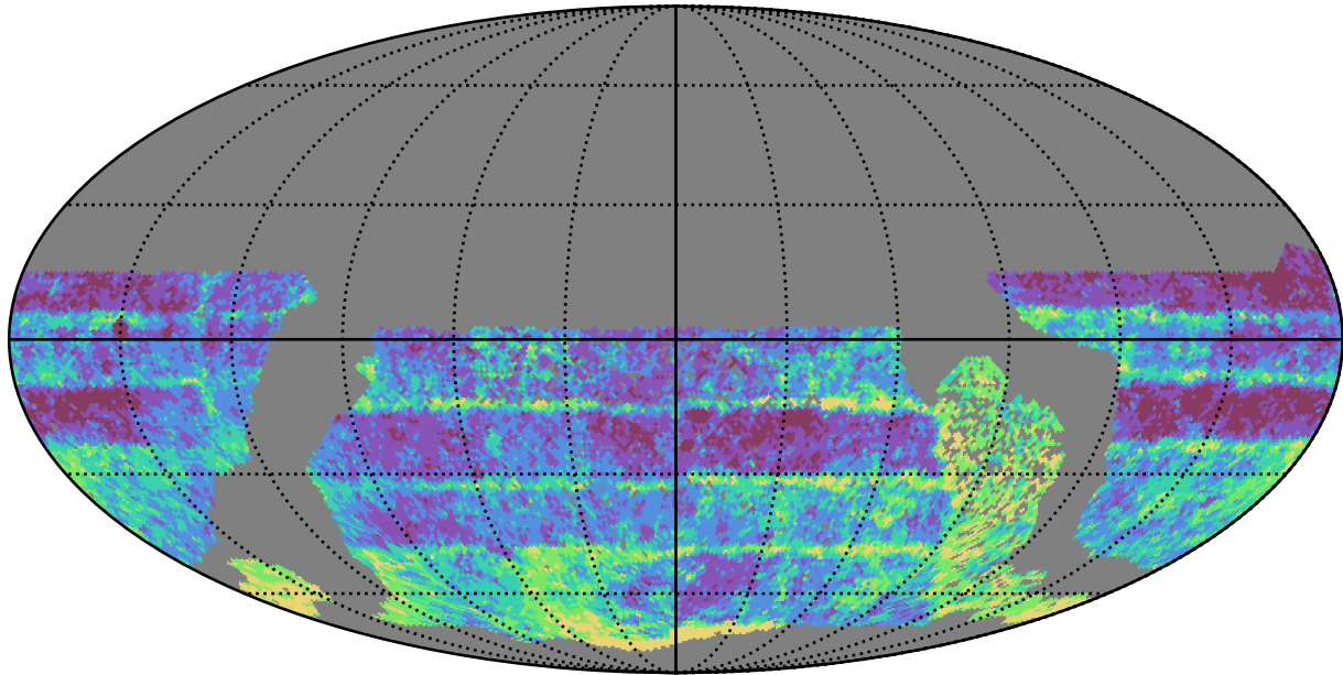
no_high_blob_v3.3_10yrs WFD r band: Median Inter-Night Gap
