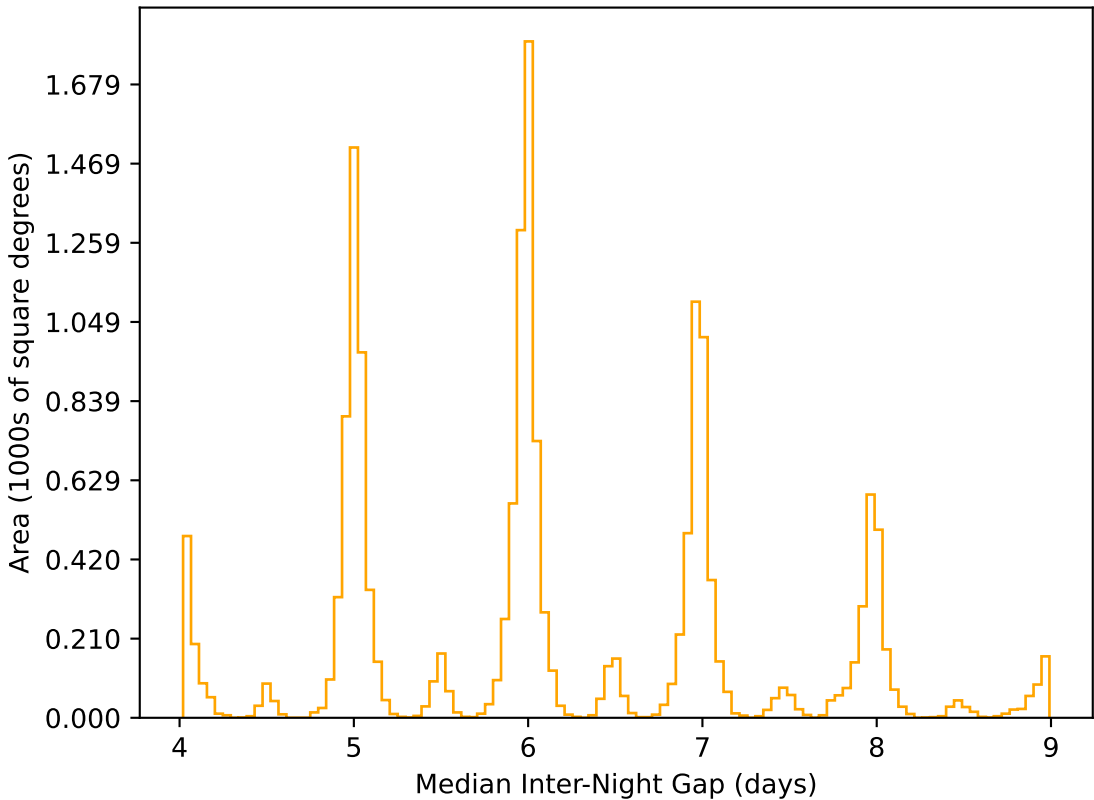
no_high_blob_v3.3_10yrs WFD r band: Median Inter-Night Gap
