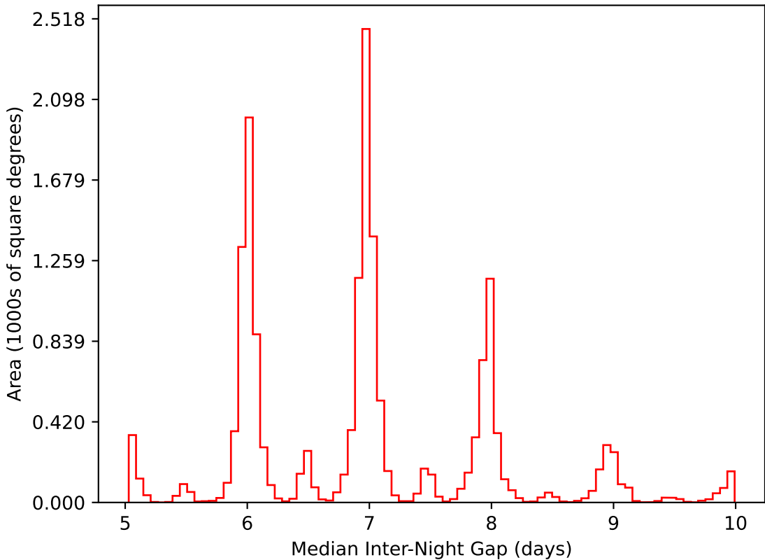
no_high_blob_v3.3_10yrs WFD i band: Median Inter-Night Gap
