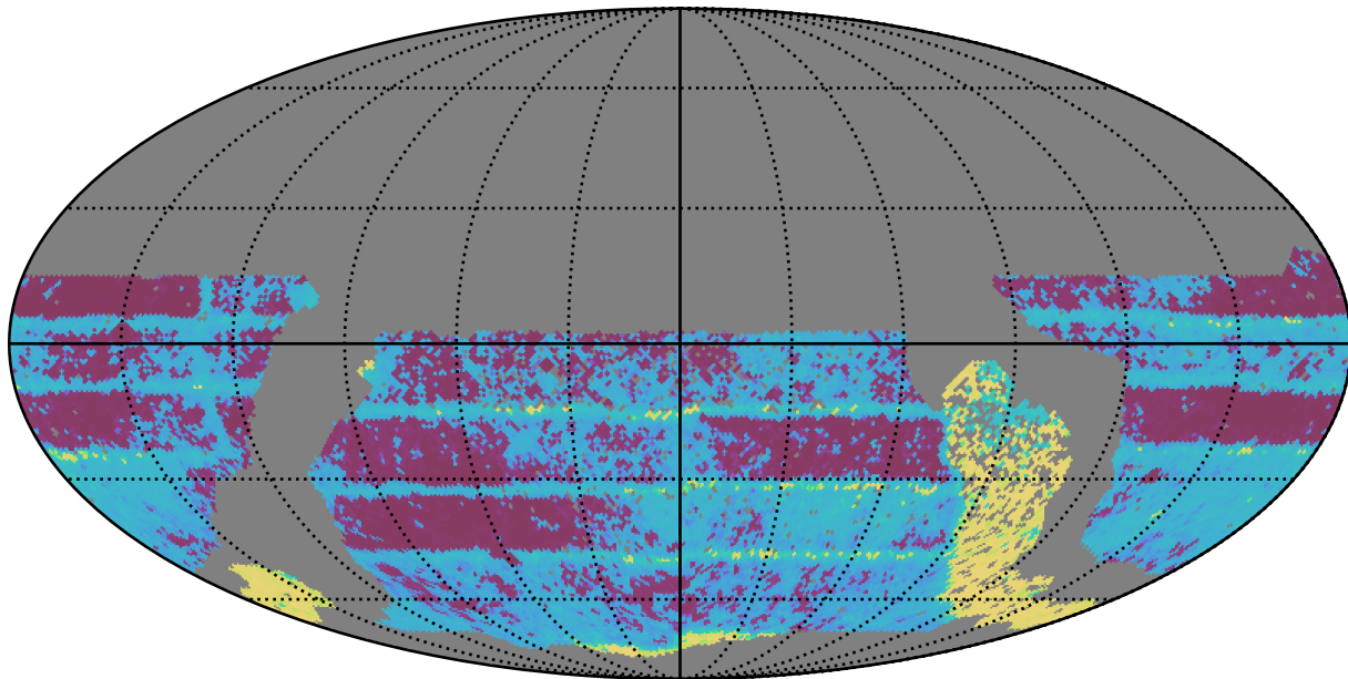
no_high_blob_v3.3_10yrs WFD all bands: Median Inter-Night Gap
