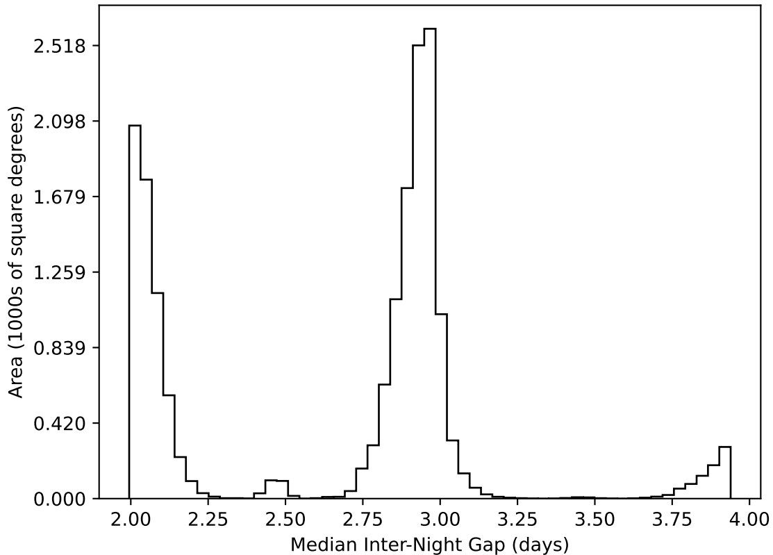
no_high_blob_v3.3_10yrs WFD all bands: Median Inter-Night Gap
