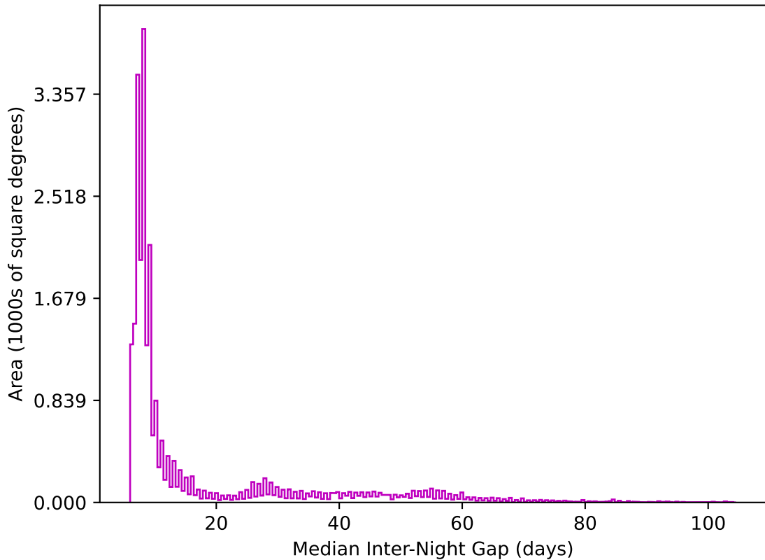
no_high_blob_v3.3_10yrs All sky z band: Median Inter-Night Gap
