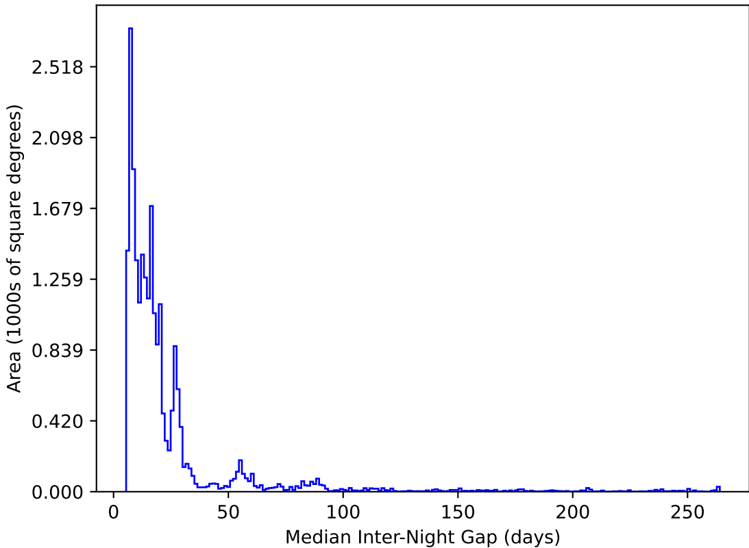
no_high_blob_v3.3_10yrs All sky y band: Median Inter-Night Gap
