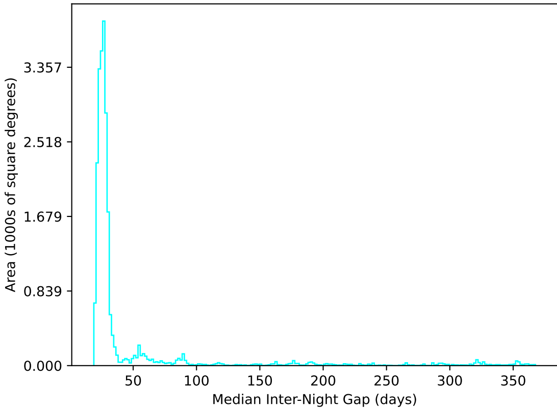
no_high_blob_v3.3_10yrs All sky u band: Median Inter-Night Gap
